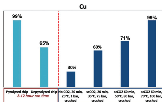
Fig. 17 Cu extraction results for pyrolyzed vs. unpyrolyzed, no CO 2 , and scCO 2 leaching solutions of PCB.
