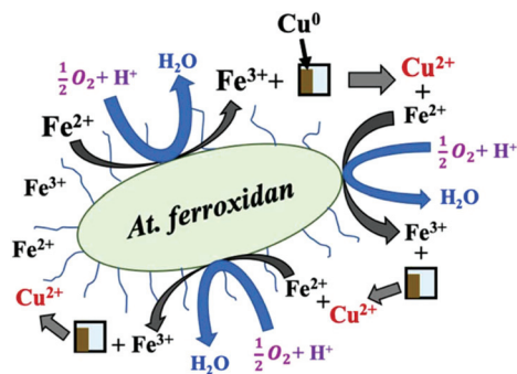
Fig. 16 The bioleaching mechanism of At. ferrooxidans in solution with shredded PCB.
